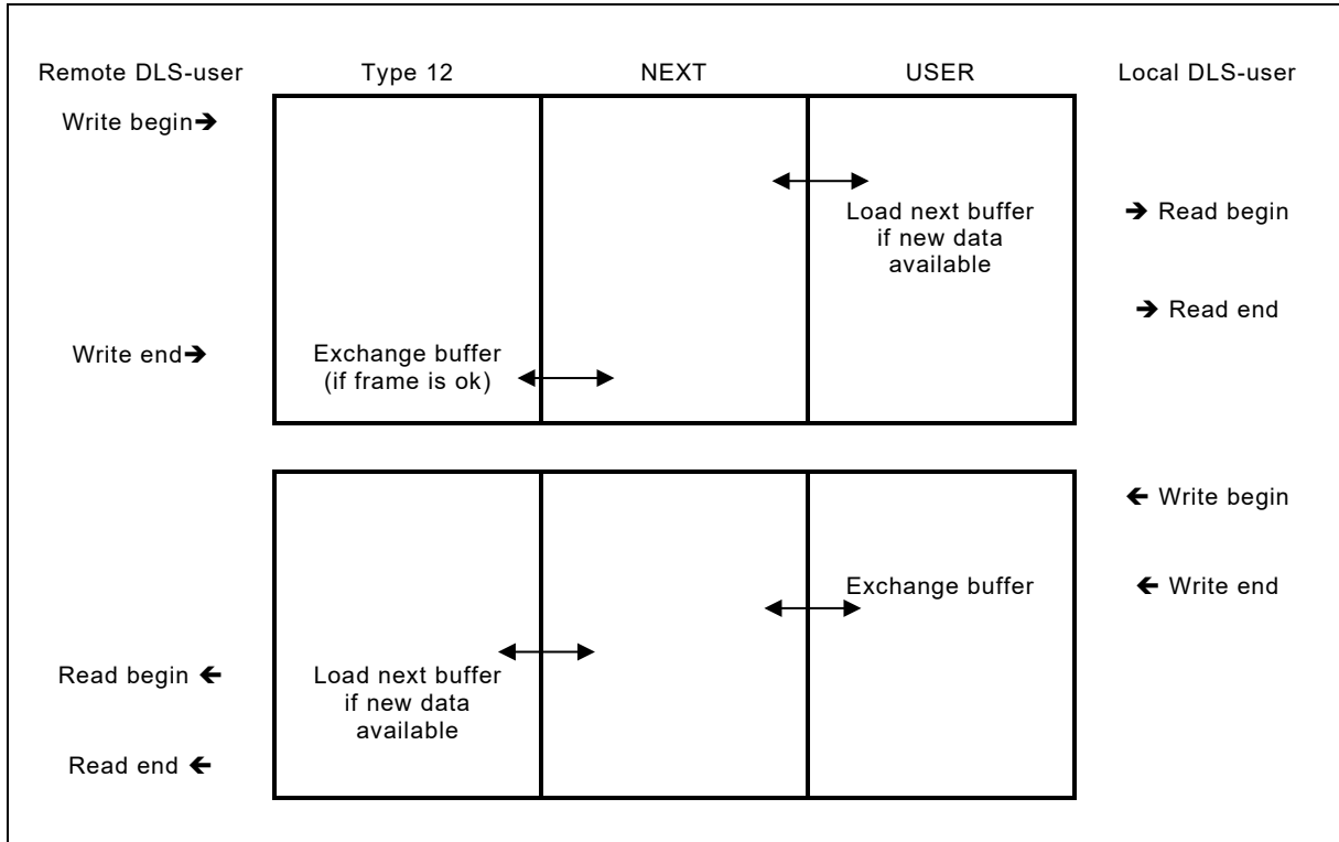
Figure 34 – SyncM buffer interaction
