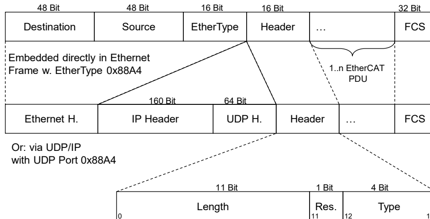
Figure 3 – Frame structure
