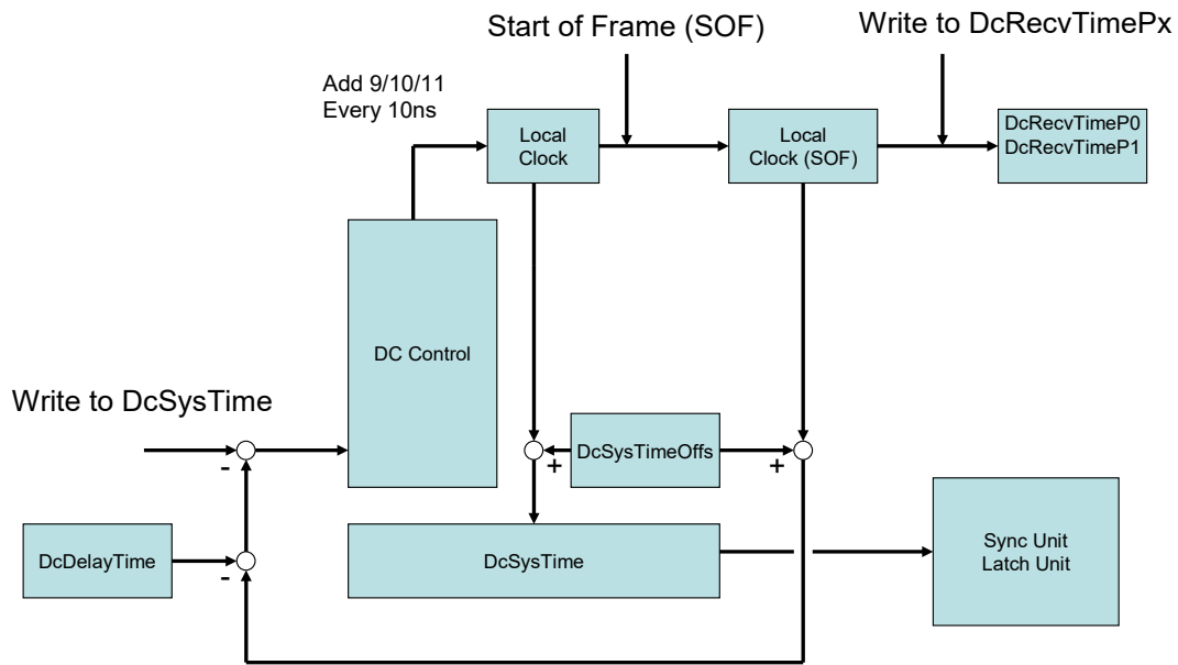
Figure 48 – Distributed clock
